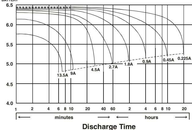
(V) Discharge Time VS. Discharge Current (25°C) FOR 6V BATTERY
